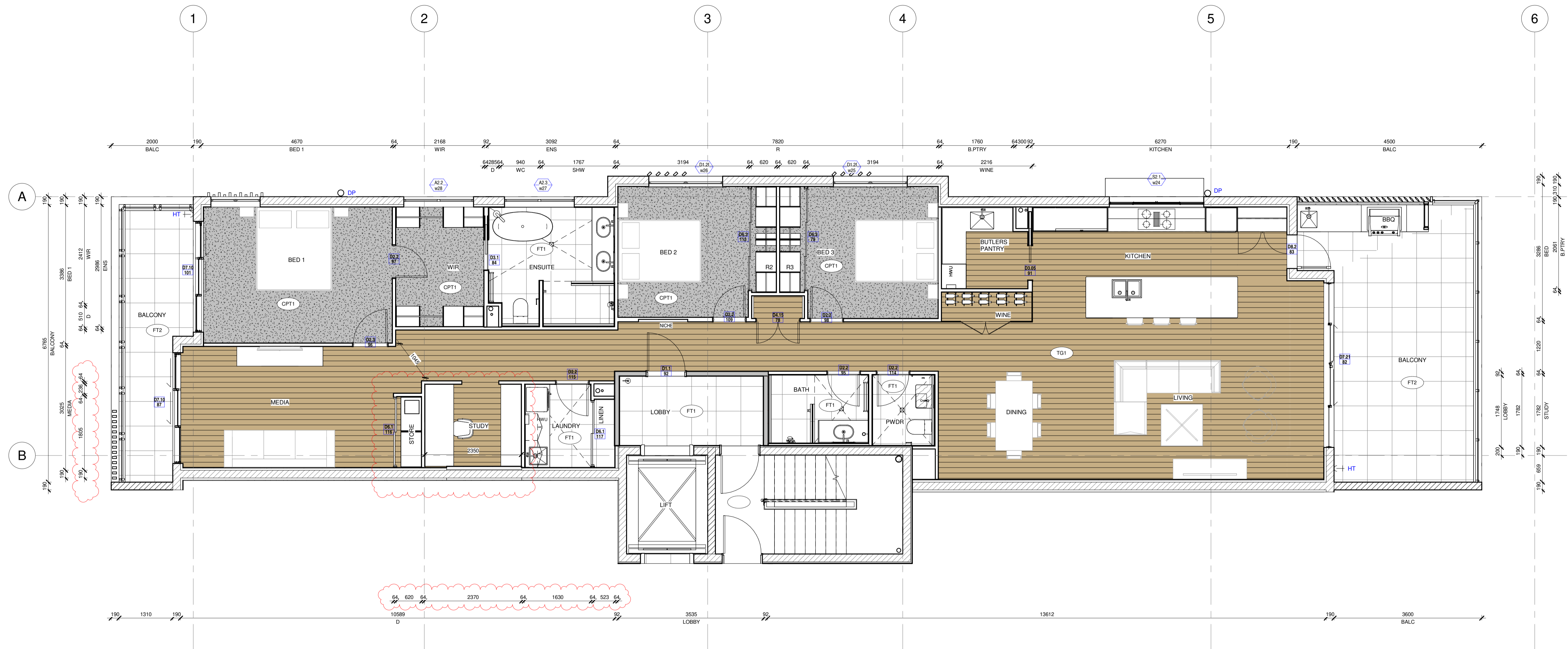
1 UNIT 5 PLAN 1 : 50 on A1 / 1 : 100 on A3
