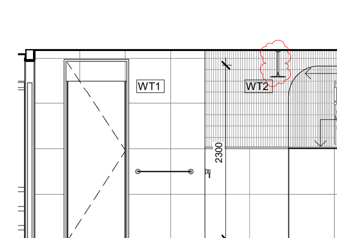
2.14 ELEVATION 1 : 50
