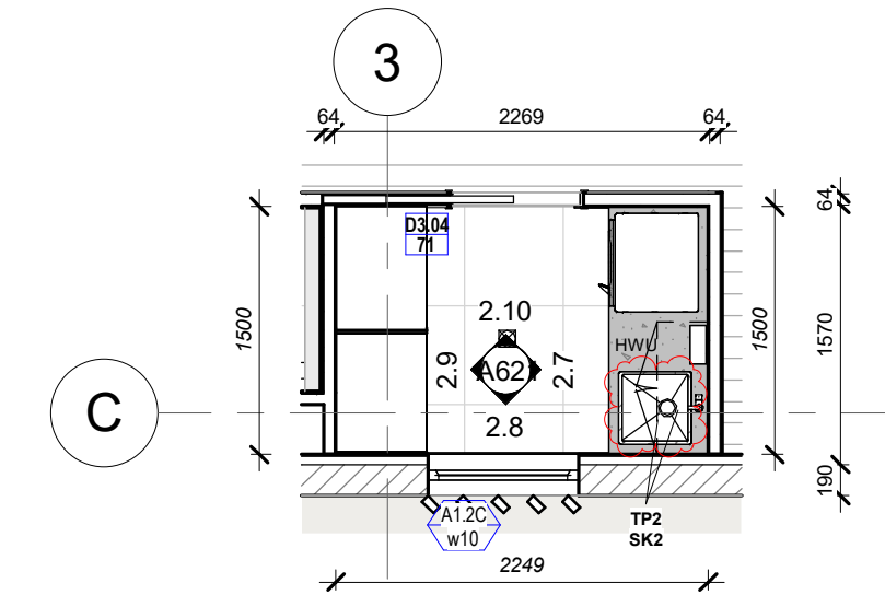
5 UNIT 2,4,6 LAUNDRY 1 : 50 on A1 / 1 : 100 on A3
