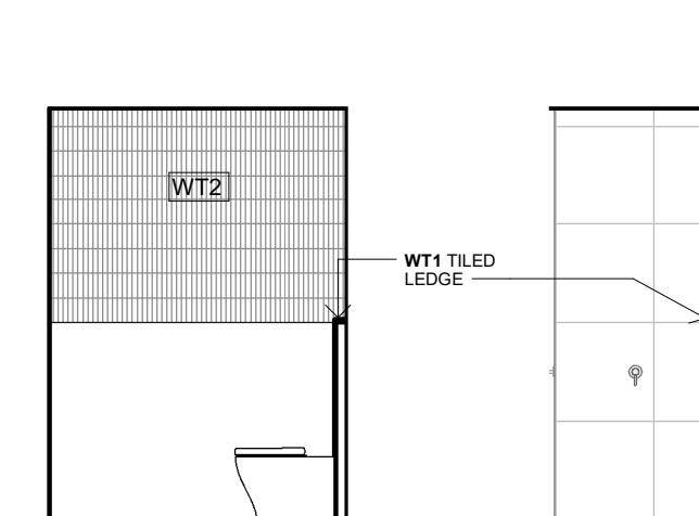
2.15 ELEVATION 1 : 50
