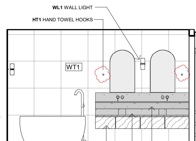
2.12 ELEVATION 1 : 50
