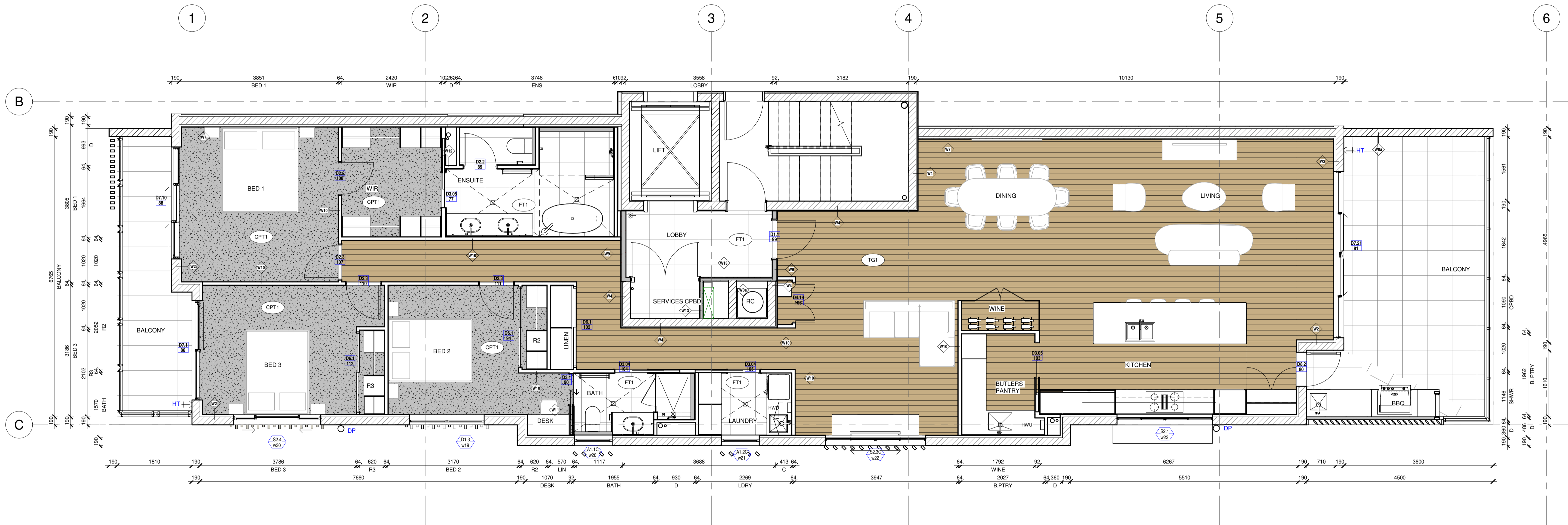
1 UNIT 4 PLAN 1 : 50 on A1 / 1 : 100 on A3
