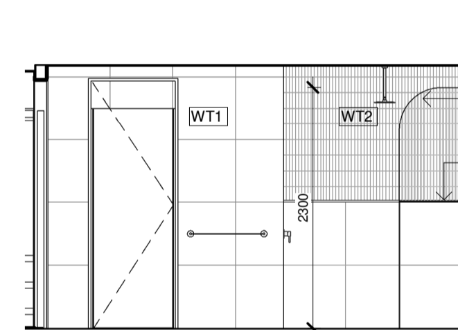
2.14 ELEVATION 1 : 50
