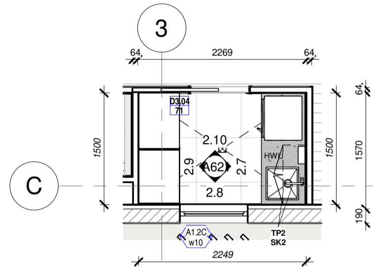
5 UNIT 2,4,6 LAUNDRY 1 : 50 on A1 / 1 : 100 on A3
