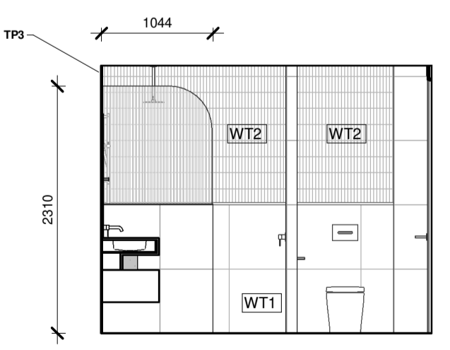
3.16 ELEVATION 1 : 50
