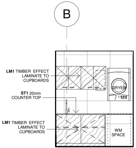
3.5 ELEVATION 1 : 50
