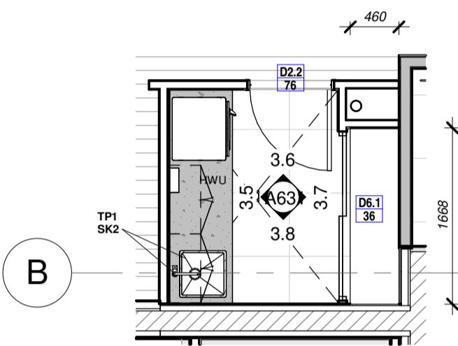
5 UNIT 3,5,7 LAUNDRY 1 : 50 on A1 / 1 : 100 on A3
