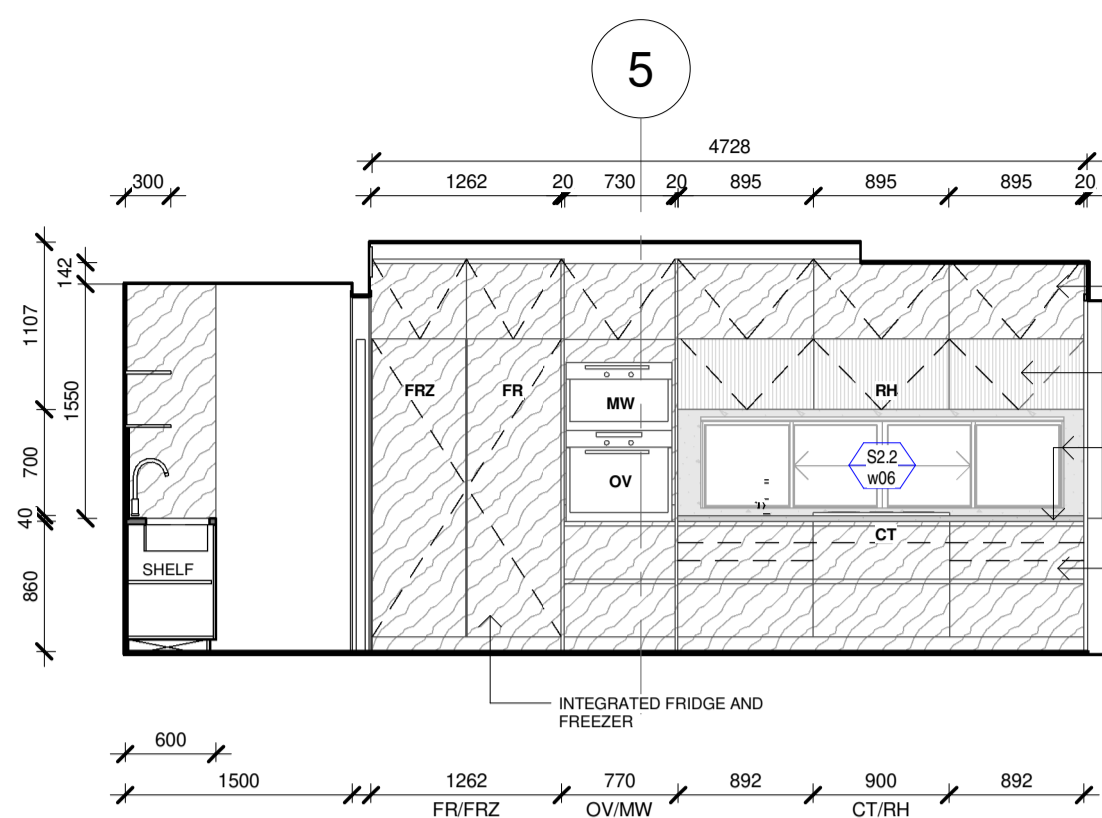
1.19 ELEVATION 1 : 50 on A1 / 1 : 100 on A3
