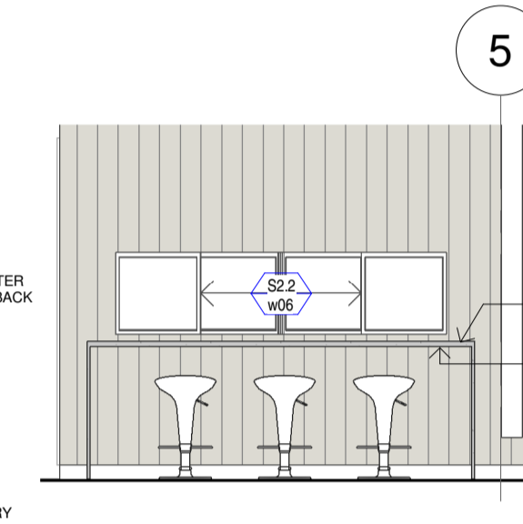
1.24 ELEVATION 1 : 50 on A1 / 1 : 100 on A3
