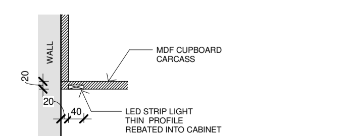
DETAIL_LED LIGHT 1 : 10
