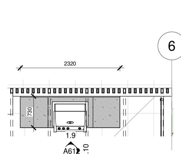
3 UNIT 1 BBQ 1 : 50 on A1 / 1 : 100 on A3
