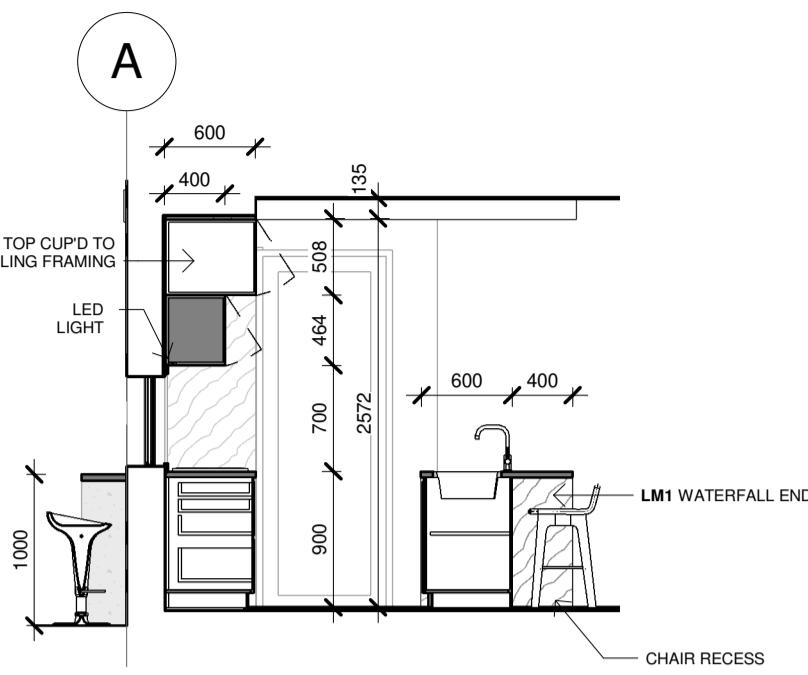
1.20 ELEVATION 1 : 50 on A1 / 1 : 100 on A3
