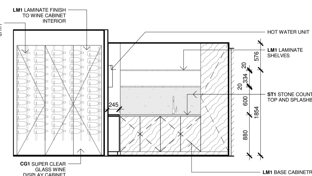
1.23 ELEVATION 1 : 50 on A1 / 1 : 100 on A3
