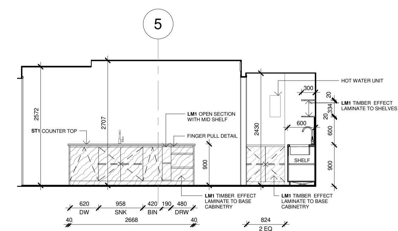
1.21 ELEVATION 1 : 50 on A1 / 1 : 100 on A3
