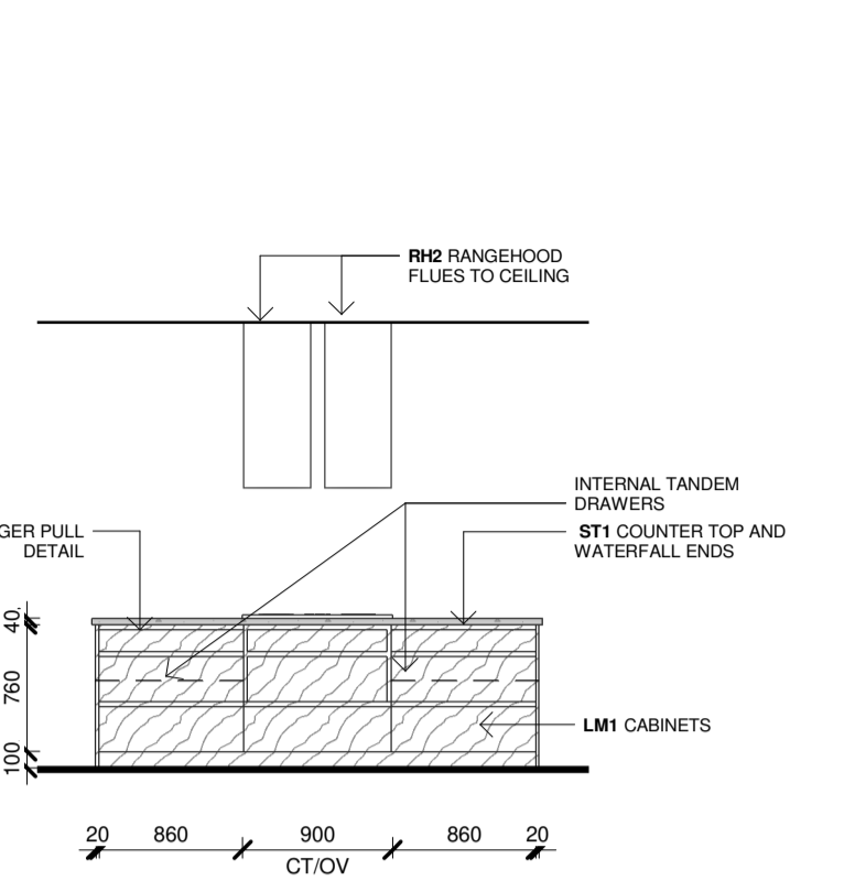
8.27 ELEVATION 1 : 50
