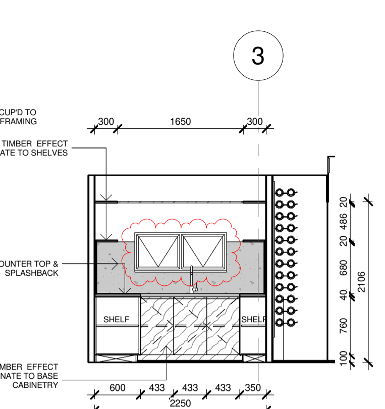
8.29 ELEVATION 1 : 50
