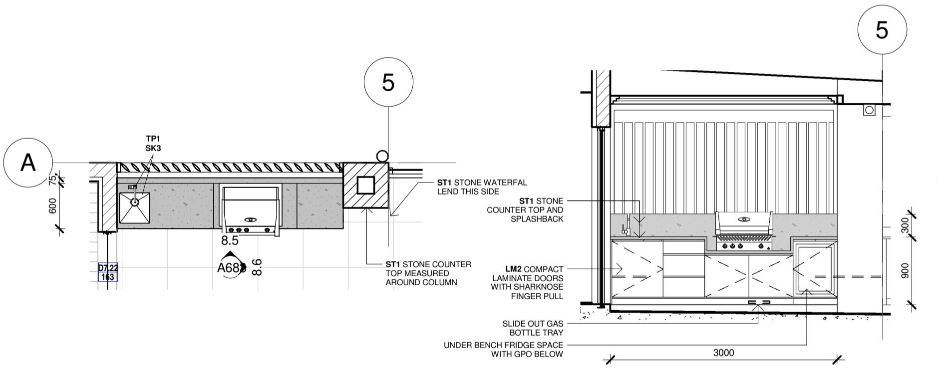
8.5 ELEVATION 1 : 50
