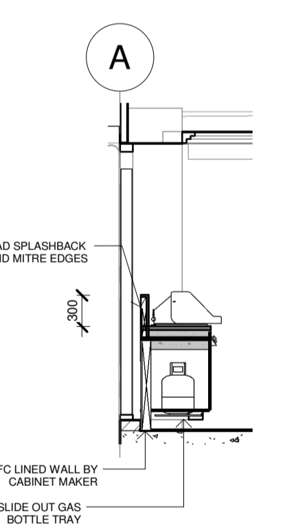
8.6 ELEVATION 1 : 50
