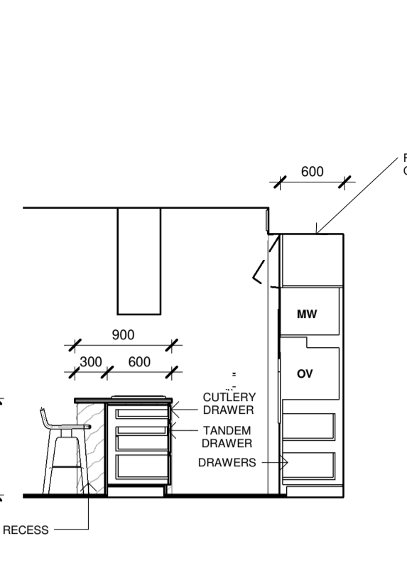
8.28 ELEVATION 1 : 50
