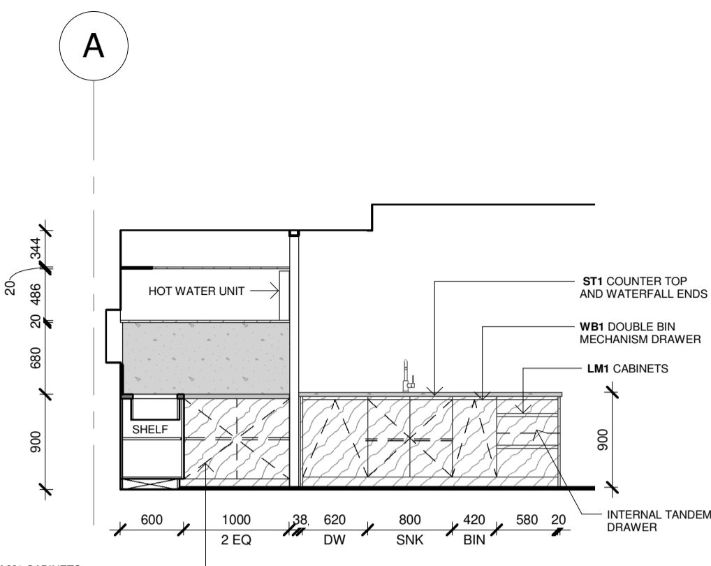
8.26 ELEVATION 1 : 50
