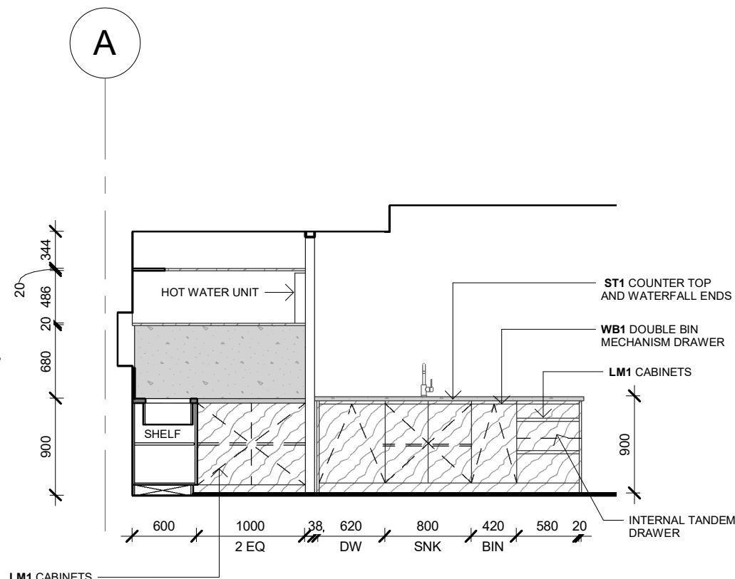
8.26 ELEVATION 1 : 50
