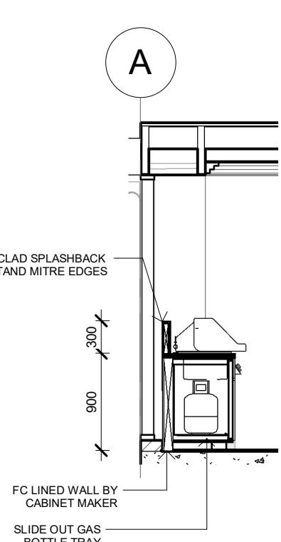
8.6 ELEVATION 1 : 50
