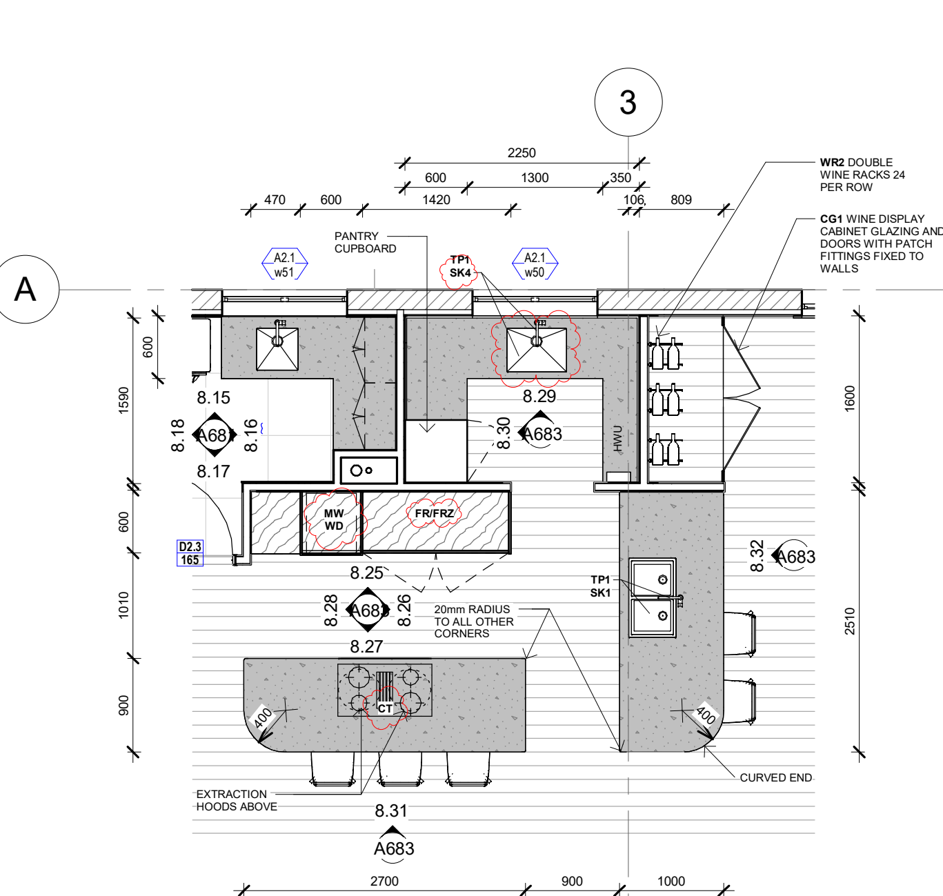
1 UNIT 8 KITCHEN 1 : 50 on A1 / 1 : 100 on A3
