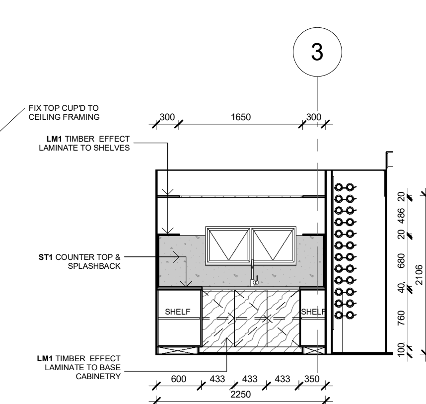
8.29 ELEVATION 1 : 50
