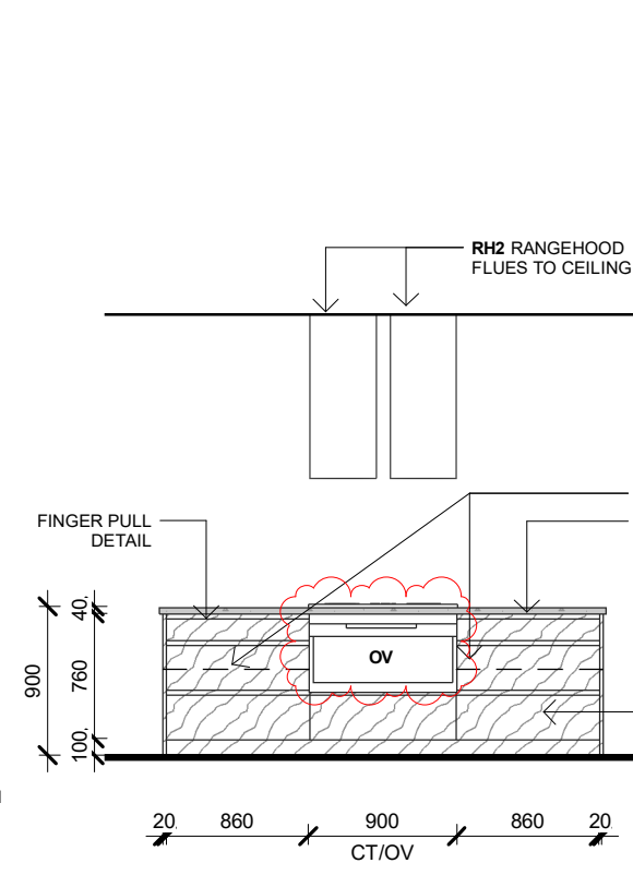
8.27 ELEVATION 1 : 50
