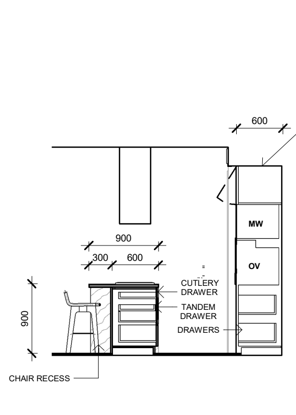
8.28 ELEVATION 1 : 50
